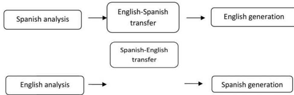
Figure 2: Transfer MT System
