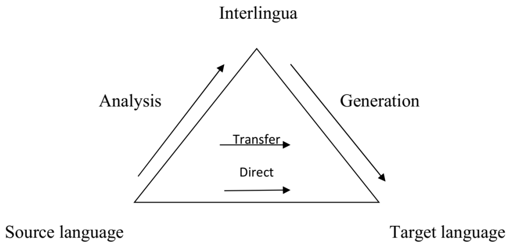
Figure 3: Difference between direct, transfer, and Interlingua MT methods
